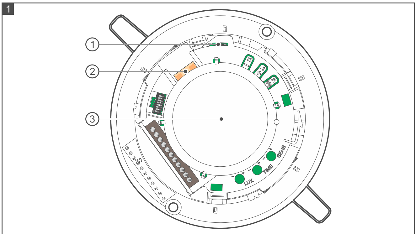
Figure 1 shows the inside of the detector after opening the enclosure.
