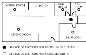
Figure 1: Installation locations for smoke & heat detectors in single-family apartments or homes with only one sleeping area
