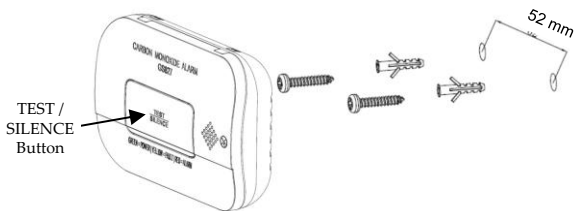
Figure 2 – Mounting
