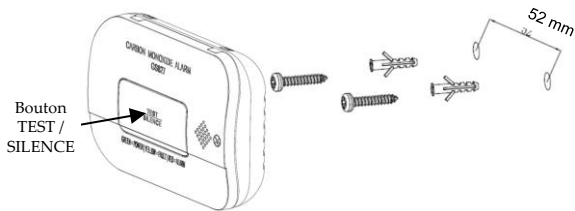
Figure 2 – Montage
