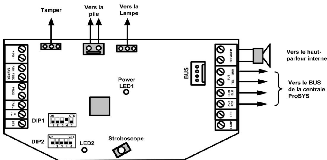
Figure 2 - Configuration BUS
