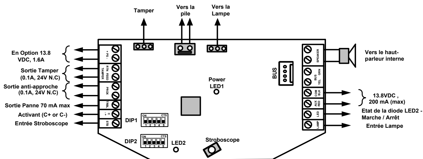
Figure 1 - Configuration autonome
