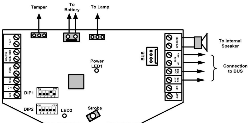
Figure 2: BUS Wiring
