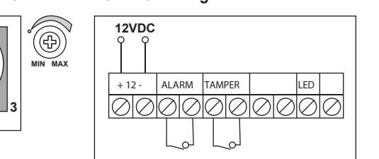
Figure 6. Terminal Wiring
