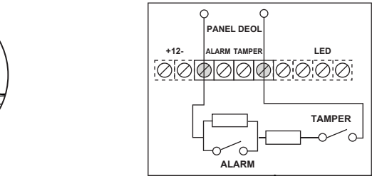
Figure 4. EOL Resistors
