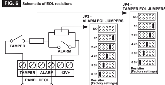
FIG. 6 Schematic of EOL resistors
